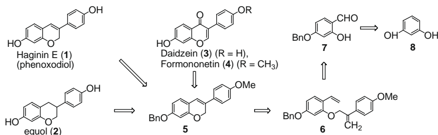
Scheme 1. Retrosynthesis of haginin E ( 1 ), equol ( 2 ), daidzein ( 3 ) and formononetin ( 4 ).
