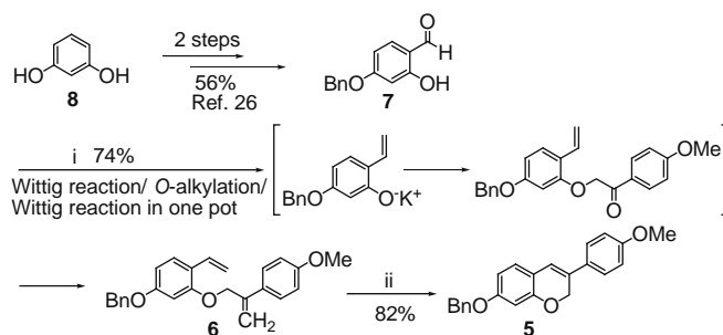
Scheme 2. Synthesis of isoflavene intermediate 5 . Reagents and conditions: (i) (a). MTPPB, t -BuOK, THF, 0 °C 2 h; (b). 2-bromo-4'-methoxyacetophenone, reflux, 1 h; c. MTPPB, t -BuOK, THF, 0 °C, 1 h. (ii) Grubbs 2nd, CH 2 Cl 2 , 40 °C, 8 h.
